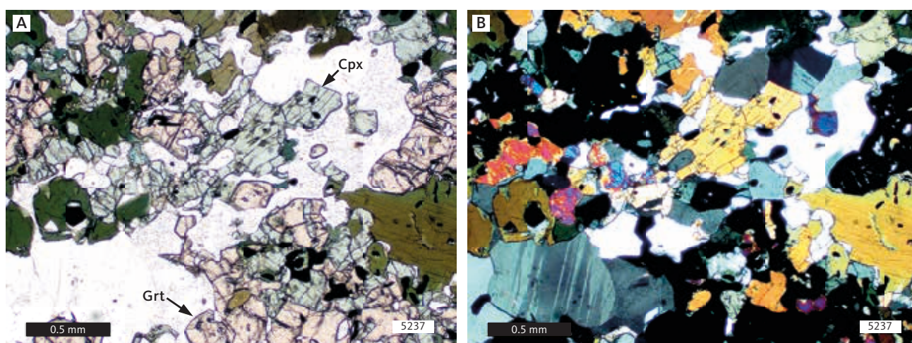
Fig. 88 Metadyke from clinopyroxene-garnet zone. A : (1 nicol) garnet ( Grt ; pink), clinopyroxene ( Cpx ; light green), and amphibole (dark green). B : is the same with X nicols. Sample 5237. North shore of inner Akulleq.
