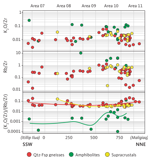
Fig. 98 Variations in K_2O and Rb in rocks hosting Kangâmiut dykes from Areas 07 to 11. Data from quartzofeldspathic gneisses, amphibolites and rocks of supracrustal origin are projected on to a c. 60 km long NNE–SSW-trending line from Maligiaq (right) to Itillip Ilua (left; see Fig. 2 for location of projection line; each unit along x-axis is c. 50 m). K_2O and Rb are normalised against an immobile element, Zr. All lithologies show unsystematic and quite scattered variations in Areas 07 and 08. From Area 09 to 11, quartzofeldspathic gneisses show a decrease in both K_2O and Rb, however since the Rb decrease is larger, the resultant K_2O:Rb increases dramatically in Area 11. Amphibolites and supracrustal gneisses show vaguely similar trends but those are based on relatively few samples. The smooth trend lines are calculated with the locally weighted least squares regression method. K_2O in wt%, Rb and Zr in ppm.
