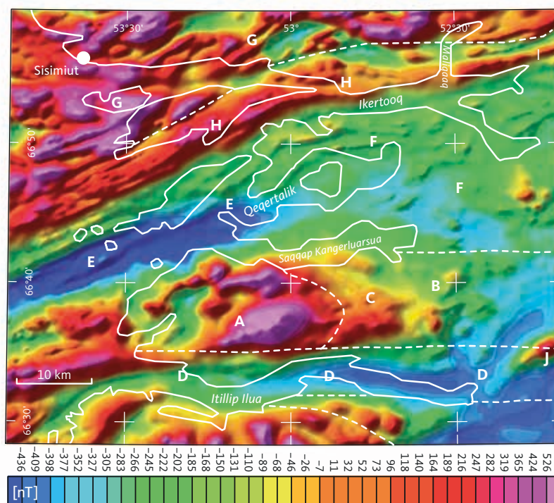
Fig. 94 Magnetic anomaly map for the Itillip Ilua – Ikertooq area (modified from Korstgård et al. 2006) showing the strong correlation between metamorphic boundaries and the magnetic signatures. A–J : magnetic anomaly centres described in Korstgård et al. 2006. The dashed white lines correspond to the metamorphic facies boundaries in Fig. 93. Within the Archaean granulite facies areas, just north and south of Itillip Ilua (A), strong magnetisations are attributed to a high content of magnetite, formed through the breakdown of hydrous mafic minerals (biotite, amphibole) during the transition from amphibolite to granulite facies. The gradual increase in magnetic intensity, from B to C to A, even conforms to this gradual prograde facies transition. The E–W-trending low magnetic anomaly, coincident with the Itilleq shear zone (D), is most likely caused by breakdown of magnetic minerals during metamorphic retrogression, from granulite facies or upper amphibolite facies (A, B, C) to epidote amphibolite facies in the shear zone (D). The post-dyke lower amphibolite facies rocks along Qeqertalik (E and F) also display low magnetic anomalies, whereas the upper amphibolite to granulite facies rocks along the Ikertooq shear zone and northwards display high magnetic anomalies (H and G). Isolated high intensity anomalies can also locally be correlated with distinct lithologies or intrusions (e.g. the anorthosite complex at J).
