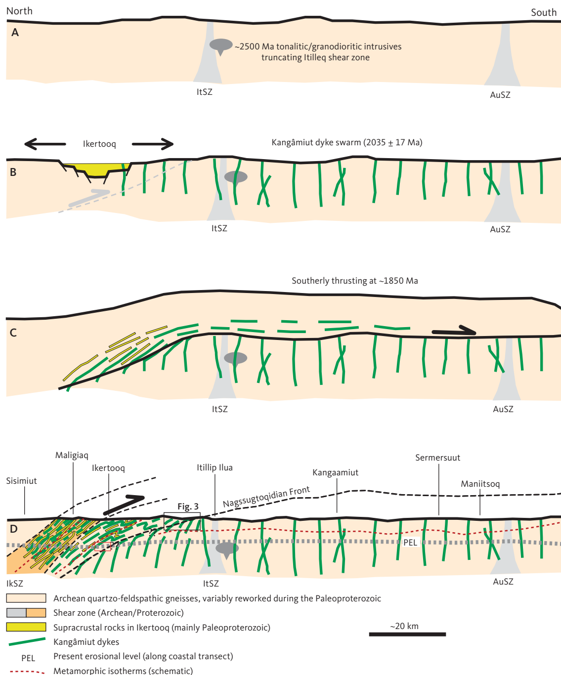
Fig. 101 Simplified cartoon illustrating the sequence of geological events described in the text for the study area between Maniitsoq and Ikertooq. A: Stable Archean crust intruded by tonalitic or granodioritic bodies at c. 2500 Ma. These units cut existing shear zones (ItSZ) of unknown, but likely Neo-archean age. IkSZ: Ikertooq shear zone. ItSZ: Itilleq shear zone. AuSZ: Aujassooq-Evighedsfjord shear zone. B: Localised crustal extension, deposition of sediments in the Ikertooq area and intrusion of the 2035 ± 17 Ma Kangâmiut dykes. C: Large-scale south-directed thrusting affects basement gneisses, sediments and dykes and causes widespread metamorphism in the footwall as far south as Maniitsoq. Metamorphic ages recorded by the dykes are around 1850 Ma. D: Strong deformation and metamorphism in the area between Itillip Ilua and Ikertooq with a northward-increasing gradient culminating in strongly sheared granulite facies rocks in Maligiaq thrust over amphibolite facies rocks. Most metamorphic ages are up to 100 Myr younger than those obtained farther south towards Maniitsoq. These ages may reflect a separate phase of tectonism or just the latest pulse in a protracted event starting with the thrusting in shown in panel C. PEL: the erosional level presently exposed along the coastal transect discussed here. Red box: approximate location of the red line shown in Fig. 93. Its relationship to the Nagssugtoqidian Front is not known nor is any implied. Geographic locations refer to locations along the coastal transect. Upper part of D , including the heavy black line , schematically represents observations farther east, closer to the Greenland ice sheet (slightly higher crustal levels due to the gentle eastward crustal tilt).
