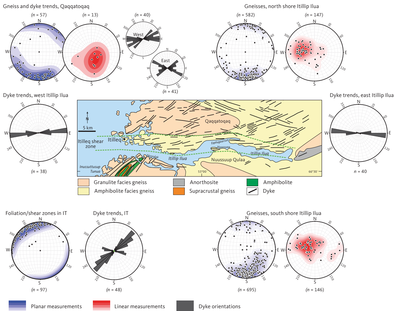
Fig. 16 Orientation plots for dykes and host gneisses in areas along and adjacent to Itilip Ilua. Data from the Inussuttusup Tunua (IT) area are from Jack (1978), the remainder are from this study. See Fig. 38 for contouring details. Planar measurements ( blue shading ) include all penetrative planar elements on outcrop scale in metadykes and host gneisses, typically a combination of mineral foliation and compositional layering (e.g. Fig. 22). Linear measurements ( red shading ) include all penetrative linear elements in metadykes and host gneisses such as mineral lineation, stretching lineation (typically quartz and feldspar aggregates), rodding, mullions and axes of minor folds (e.g. Fig. 23). Green dashed lines : denote the Itilleq shear zone.
