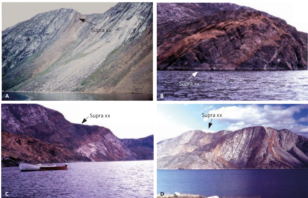
Fig. 39 Field examples of supracrustal sequences ( Supra xx ). A : Steeply NW-dipping supracrustal sequence in the south-easternmost part of Qeqertalik. Height of cliff c. 150 m. B : Moderately NW-dipping supracrustal sequence along east shore of Avalleq. Height of cliff in foreground c. 20 m. C : Shallowly NW-dipping supracrustal sequence along east shore of Avalleq. D : Steeply NW-dipping supracrustal sequence in Avalleq. Height of cliff c. 250 m.
