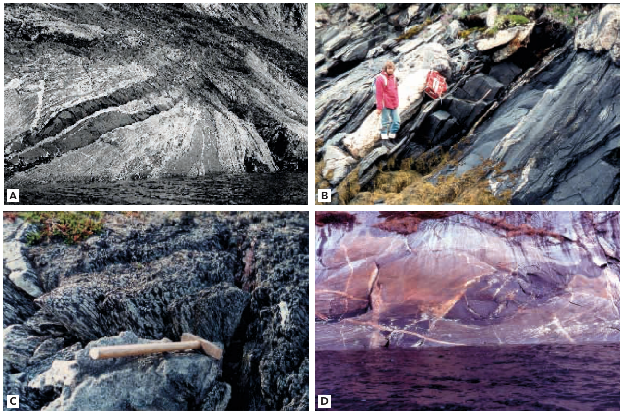
Fig. 42 Field examples from north-east shore of Avalleq. A: Banded gneiss with older mafic bodies conformably cut by c. 1 m wide Kangâmiut metadykes. B: Conformable metadyke in gneiss. C: Stretching lineation in metadyke defined by plagioclase aggregates. Hammer is 40 cm. D: Disrupted metadyke in gneiss. Large pod is c. 10 m long.
