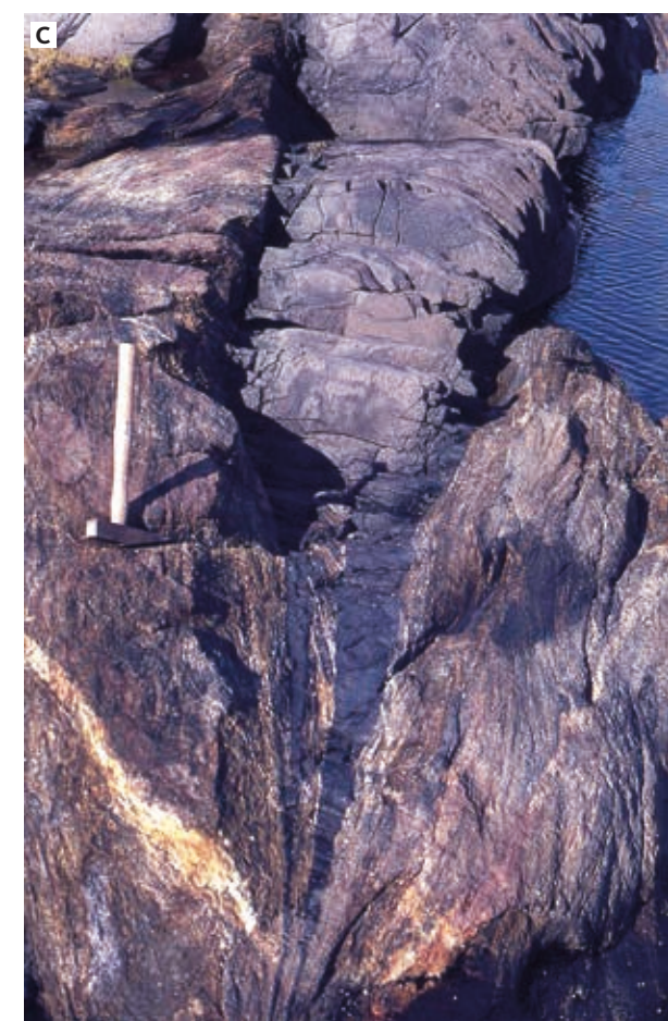
Fig. 30 Intrusive features in podded dykes from the north shore of Itillip Ilua. A: Field sketch of 20 m wide Kangâmiut dyke that over 20 m narrows to a couple of centimetre-wide strands. Reproduced from Korstgård (1980). B: Field sketch of 50 m wide Kangâmiut dyke pod at the end of which is an intricate network of interconnected apophyses that are discordant to the host rock foliation and entirely undeformed. This suggests that the thinning of the pod is a primary feature rather than the result of deformation. From Korstgård (1980). C: Delicate discordant features preserved along thin dyke strands at tip of pod in Kangâmiut dyke. Hammer is 40 cm.
