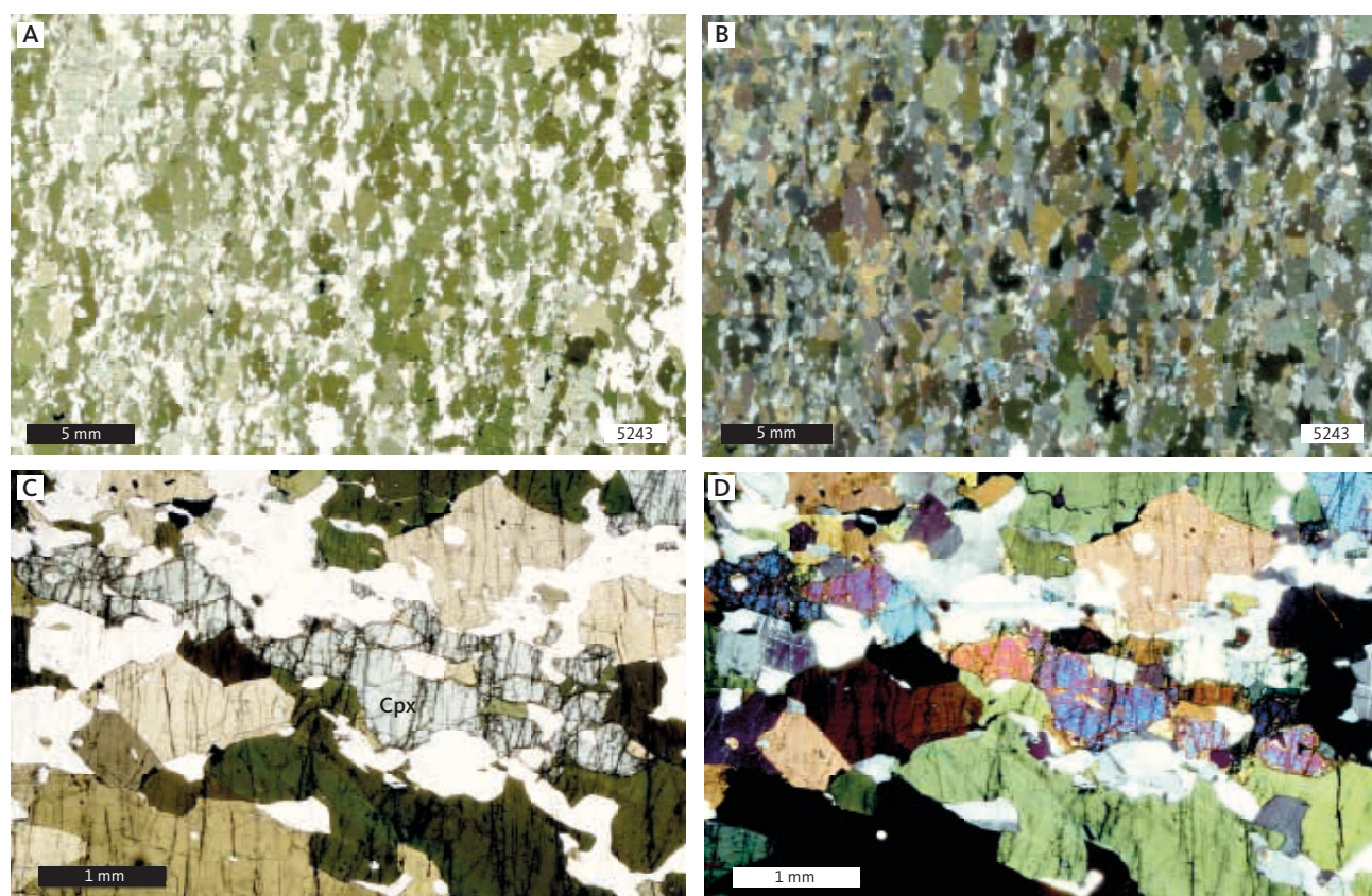
Fig. 87 Upper amphibolite facies metadyke. A (1 nicol), B (X nicols): good foliation with amphibole (dark green) and clinopyroxene (light green). C (1 nicol), D (X nicols): clinopyroxene in centre. Sample 5243. North shore of outer Akulleq.
