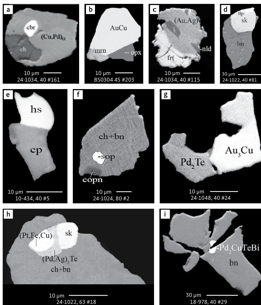
Fig. 31 BSE images of rare intermetallic compounds of precious metals in polished monolayer thin sections of HS concentrates. The rare occurrence of these phases illustrates parageneses buffered by very localised geochemical conditions. Table 3 provides formulae for the precious metal minerals. Formulae for common rock-forming minerals and base metal sulphides are found in Appendix 1. Formulae are given here for rare minerals that are not listed in Table 3 or Appendix 1. Abbreviated names of minerals, compounds and alloys are as follows: cbr : cabriite ( \text{Pd}_2\text{CuSn} ). mrn : merenskyite ( \text{PdTe}_2 ). nld : naldrettite ( \text{Pd}_2(\text{Sb,Sn}) ). tlp : telargalpalite ( (\text{Pd,Ag})_2\text{Te} ). hs : hessite ( \text{Ag}_2\text{Te} ). sop : sopcheite ( \text{Ag}_4\text{Pd}_3\text{Te}_4 ). fr : froodite ( \text{PdBi}_2 ). Pd 2 Te , (Pd,Ag) 2 Te and Pd 2 CuTeBi : unnamed compounds. sk : skaergaardite. AuCu : tetra auricupride. (Cu,Pd) α : unnamed compound. (Au,Ag) : native gold. Au 3 Cu : unnamed compound. (Pt,Fe,Cu) : alloy of Pt, Fe and Cu. bn : bornite. cp : chalcopryrite. copn : cobaltian pentlandite. ch : chalcocite. opx : orthopyroxene. Grain numbers and scales included in the images.
