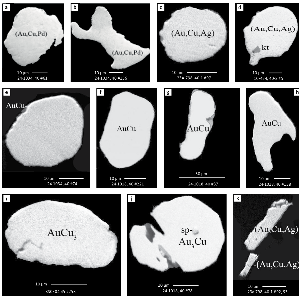
Fig. 24 BSE images of free grains of Au and Cu minerals in monolayer polished thin sections of HS concentrates. Abbreviated names of minerals, compounds and alloys are as follows: AuCu : tetra-aurocupride. AuCu 3 : aurocupride. Au 3 Cu : unnamed alloy. (Au,Cu,Pd) , (Au,Cu,Ag) : alloys of Au, Cu, Pd and Ag. sp : sperrylite. kt : kotulskite. Table 3 provides formulae for the precious metal minerals. Formulae for common rock-forming minerals and base metal sulphides are found in Appendix 1. Grain numbers and scales included in the images.
