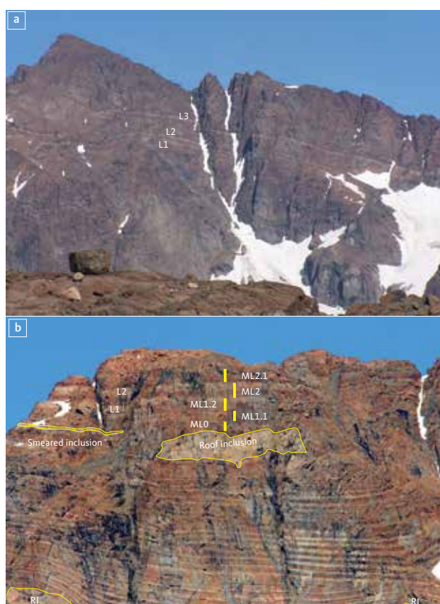
Fig. 2 The leucogabbro layers (L1, L2 and L3) of the Triple Group on Wagertoppen. a: L1 to L3 on the western face of Wagertoppen (1277 m). Large sunken blocks of roof gabbro (RI: roof inclusions) disturb the layering. In some cases, the layering drapes around the blocks (photo: M.B. Holness). b: L1 and L2 on the NW face of Wagertoppen with distinct modal layering of the zebra-banded zone at its base. Several sunken roof blocks are fully preserved or smeared (photo: J.C.Ø. Andersen). Macro-rhythmic layers ML0 to ML2.1 with leucogabbro tops are indicated by the yellow bars. The upper metres of ML0 host the Pd5 mineralisation level, and ML2.1 hosts Pd1/Au (modified from Nielsen et al. 2019a).
