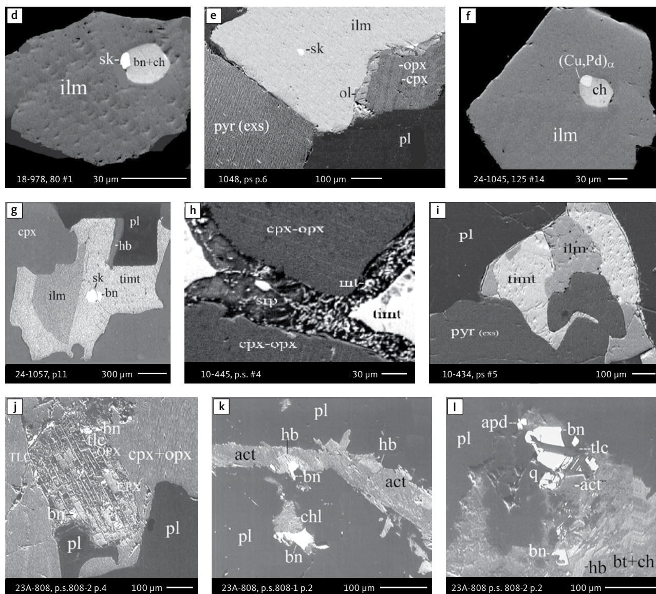
Fig. 6 (Continued) Backscattered electron (BSE) images of the petrographic relations between rock-forming silicates, oxides, sulphides and PGE phases in polished thin sections (panels a–c, e, g–i) and polished monolayer thin sections of HS concentrates (panels d, f). a–g : samples from the central part of the intrusion (drill cores 90-18, 90-24 and ToF). h–i : samples from more marginal parts of the intrusion (drill cores 90-10 and 90-23A). Abbreviated names of minerals, compounds and alloys are as follows: bn and BN : bornite. ch and cc : chalcocite. cpx and CPX : clinopyroxene. opx and OPX : orthopyroxene. pyr (exs) : cpx-opx exsolution. pl and PL : plagioclase (includes pl I with An_{38-42} and pl II with An_{82} ). timt : titaniferous magnetite. ilm : ilmenite. ol : olivine. mt : magnetite. hb : hornblende. act : actinolite. bt : biotite. q : quartz. srp : serpentine. tlc and TLC : talc. chl : chlorite. sk and SK : skagerrite. (Cu,Pd) \alpha : Pd-Cu alloy. apd : arsenopalladinite. Grain numbers and scales included in the images. Table 3 provides standard formulae for the precious metal minerals. Formulae for common rock-forming minerals and base metal sulphides are found in Appendix 1.
