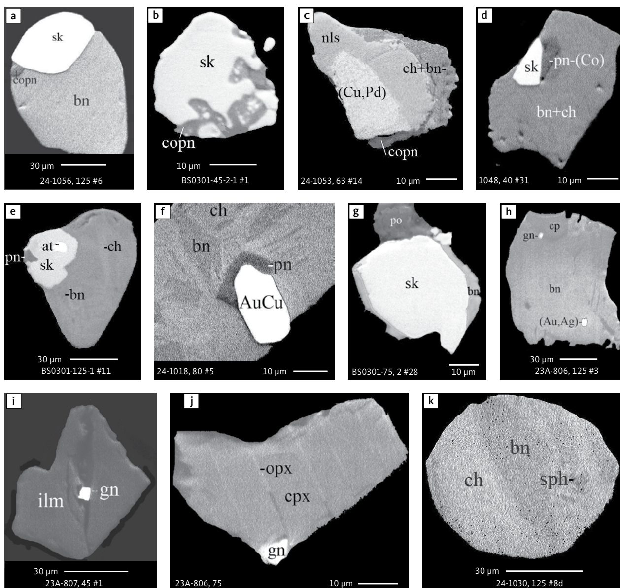
Fig. 8 BSE images of rare minerals in polished monolayer thin sections. Table 3 provides formulae for the precious metal minerals. Formulae for common rock-forming minerals and base metal sulphides are found in Appendix 1. Formulae are given here for rare minerals that are not listed in Table 3 or Appendix 1. Abbreviated names of minerals, compounds and alloys are as follows: copn and pn-(Co) : cobaltian pentlandite (panels a–d). pn : pentlandite (panels e–f). po : hexagonal pyrrhotite (panel g). gn : galena (panels h–j). sph : sphalerite (panel k). ZnS : sphalerite (panel l). CdS : greenockite/hawleyite (panels m, n). cls : clausthalite (PbSe) (panel o). aspy : arsenopyrite (panel p). spn : thiospinel group, carrollite (Cu(Co,Fe,Ni) 2 S 4 ) (panel q). atc : atacamite (Cu 2 Cl(OH) 3 ) (panel r). sk : skærvaardite (panels a, b, e, g, i). (Cu,Pd) : Cu-Pd alloy (panel c). nls : nielsenite (PdCu 3 ) (panel c). at : atokite (Pd 3 Sn) (panel e). AuCu : tetra-aurocupride (panels f, q). (Au,Ag) : native gold (panel h). Pd 3 Ag 2 S : coldwellite (panel n). vsl : vasilite ((Pd,Cu) 16 S 7 ) (panel r). bn : bornite. ch : chalcocite. cp : chalcopyrite (panels h, o). cpx : clinopyroxene (panel j). opx : orthopyroxene (panels j, q). pl : plagioclase (panel q). ilm : ilmenite (panels i, p). sk : skærvaardite (panel l). Grain numbers and scales included in the images.
