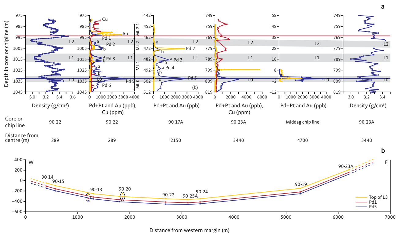
Fig. 4 Correlation between elemental concentrations and lithology of host gabbro in the Skaergaard PGE-Au Mineralisation. a: PGE, Au and Cu concentrations and density profiles of the Skaergaard PGE-Au Mineralisation. The correlations demonstrate the continuity of layering, mineralisation levels and lateral variations in elemental distributions. Blue: PGE (Pd+Pt); yellow: Au, and red: Cu. From left to right: density profile and (Pd+Pt), Au and Cu in the centrally located drill core 90-22, 25 cm bulk-rock samples; (Pd+Pt) and Au in drill core 90-17A located 1150 m from the western margin, 1 m bulk-rock samples; (Pd+Pt), Au and Cu in drill core 90-23A located 900 m from the eastern margin of the intrusion; and (Pd+Pt), Au and density profile in the Middag chip line profile, c. 5 km N of the central mineralisation (locations in Fig. 1). Grey shading indicates the elevation of leucogabbro layers L0 , L1 and L2 of the Triple Group (see Nielsen et al. 2015, 2019a for further information). Modified from Nielsen et al. 2019a. b: Cross-section of the Skaergaard intrusion (core locations in Fig. 1b; for locations of cores not used in this study see Nielsen et al. 2019a) with projected mineralisation intersects (to scale). Elevations of Pd5 ( blue ) and Pd1 ( red ) mineralisation levels and leucogabbro layer L3 ( yellow ) are relative to sea level. The profile only includes data from drill cores Pd5, Pd1 and L3. Mineralisation levels and the lithological layering are concordant across the 7000 m wide and >600 m deep bowl-shaped succession of MZ gabbros. Slightly modified from Nielsen et al. (2019a).
