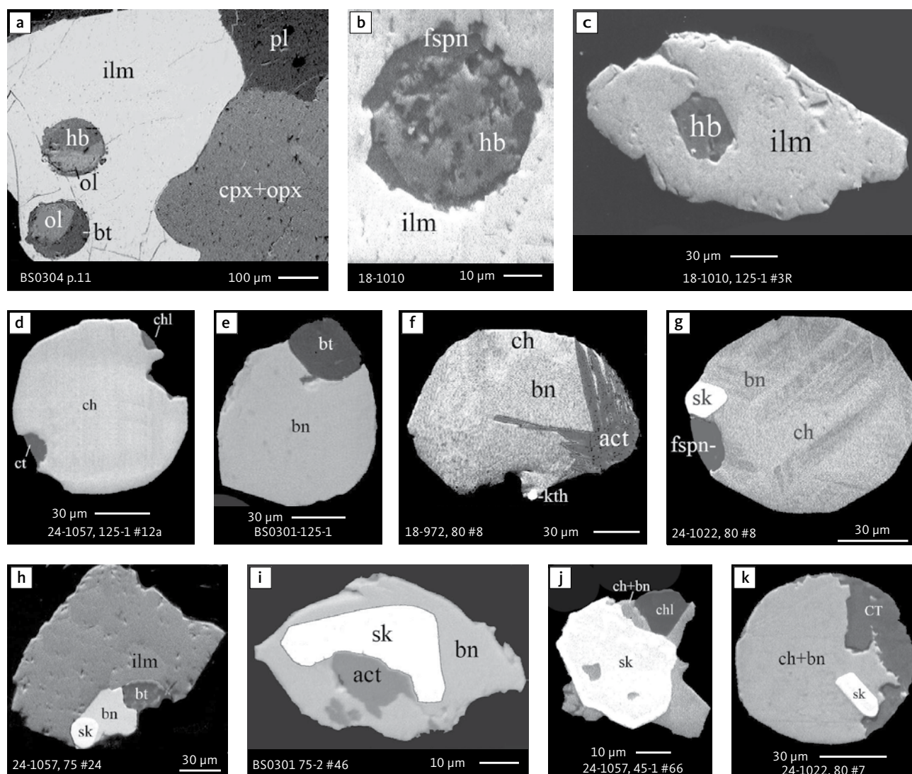
Fig. 14 BSE images of silicate globules in ilmenite and examples of hydrous silicates coexisting with sulphides and skargaardite in polished thin sections and polished monolayer thin sections of gabbroic host and in heavy mineral HS concentrates. Table 3 provides formulae for the precious metal minerals. Formulae for common rock-forming minerals and base metal sulphides are found in Appendix 1. Abbreviated names of minerals, compounds and alloys are as follows: ilm : ilmenite. cpx : clinopyroxene. opx : orthopyroxene. ol : olivine. hb : hornblende. bt : biotite. act : actinolite. fspn : ferrosaponite. chl : chlorite. ct and CT : calcite. bn : bornite. ch : chalcocite. sk : skargaardite. kth : keithconnite. pl : plagioclase. Grain numbers and scales included in the images.
