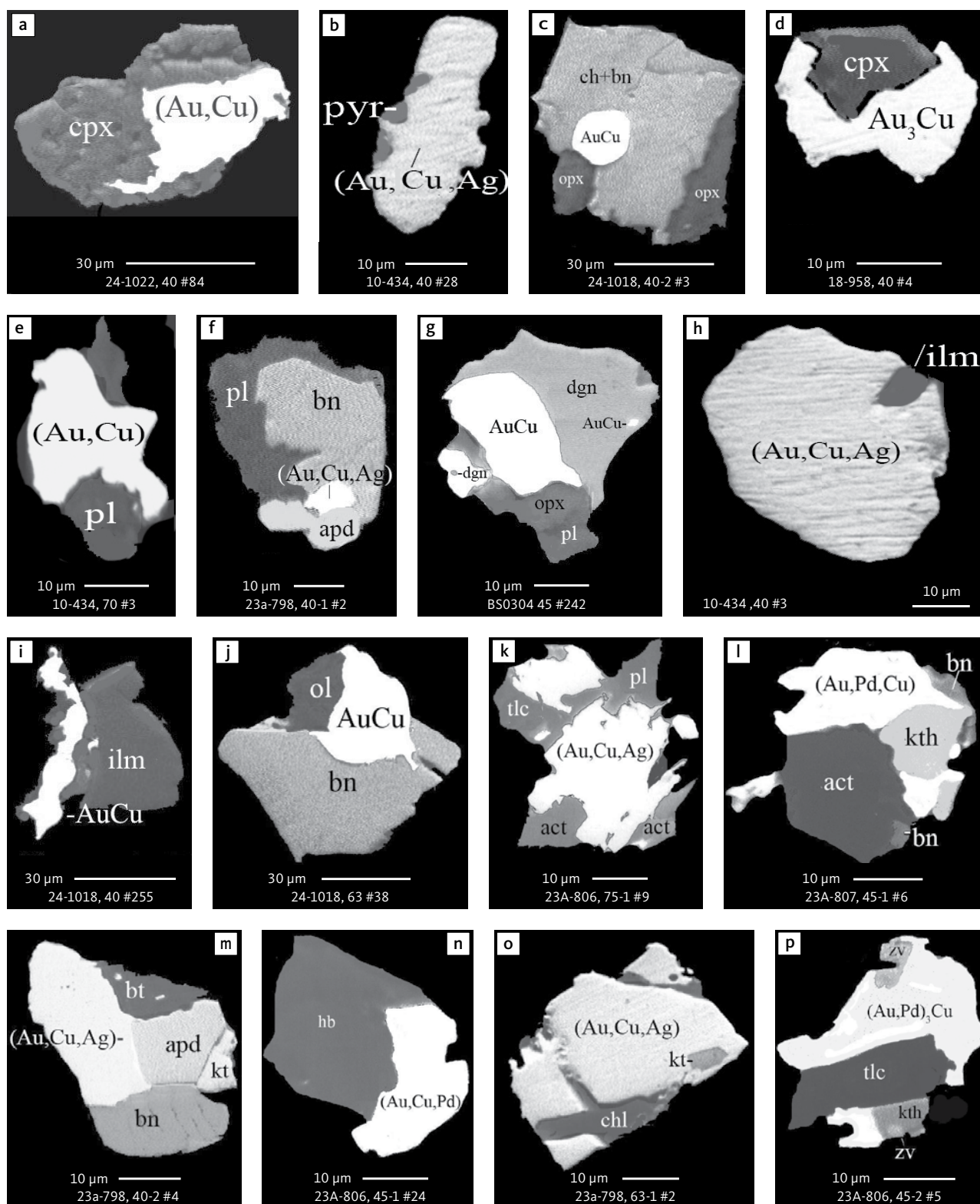
Fig. 27 Relationship between Au and Cu minerals and rock-forming minerals of the gabbroic host in polished monolayer thin sections of HS concentrates. Note that Au-Cu phases in general coexist with 'dry' parageneses in the centre of the intrusion (samples from drill cores 90-24 and 90-18, and bulk sample BS0304), and with hydrous silicate parageneses near the margins (samples from drill core 90-10 and 90-23A). Table 3 provides formulae for the precious metal minerals. Formulae for common rock-forming minerals and base metal sulphides are found in Appendix 1. Grain numbers and scales included in the images. Abbreviated names of minerals, compounds and alloys are as follows: AuCu : tetra-aurocupride. (Au,Cu) , (Au,Cu,Ag) , (Au,Pd,Cu) , (Au,Cu,Pd) : alloys of Au, Cu, Pd and Ag. Au 3 Cu and (Au,Pd) 3 Cu : unnamed compounds. apd : arsenopalladinite (Pd 3 As 2 ). zv : zvyagintsevite (Pd 3 Pb). kth : keithconnite (Pd 3-x Te). kt : kotulskite (PdTe). cpx : clinopyroxene. opx : orthopyroxene. pyr : pyroxene. pl : plagioclase. ol : olivine. ilm : ilmenite. hb : hornblende. act : actinolite. bt : biotite. chl : chlorite. tlc : talc. bn : bornite. ch : chalcocite. dgn : digenite.
