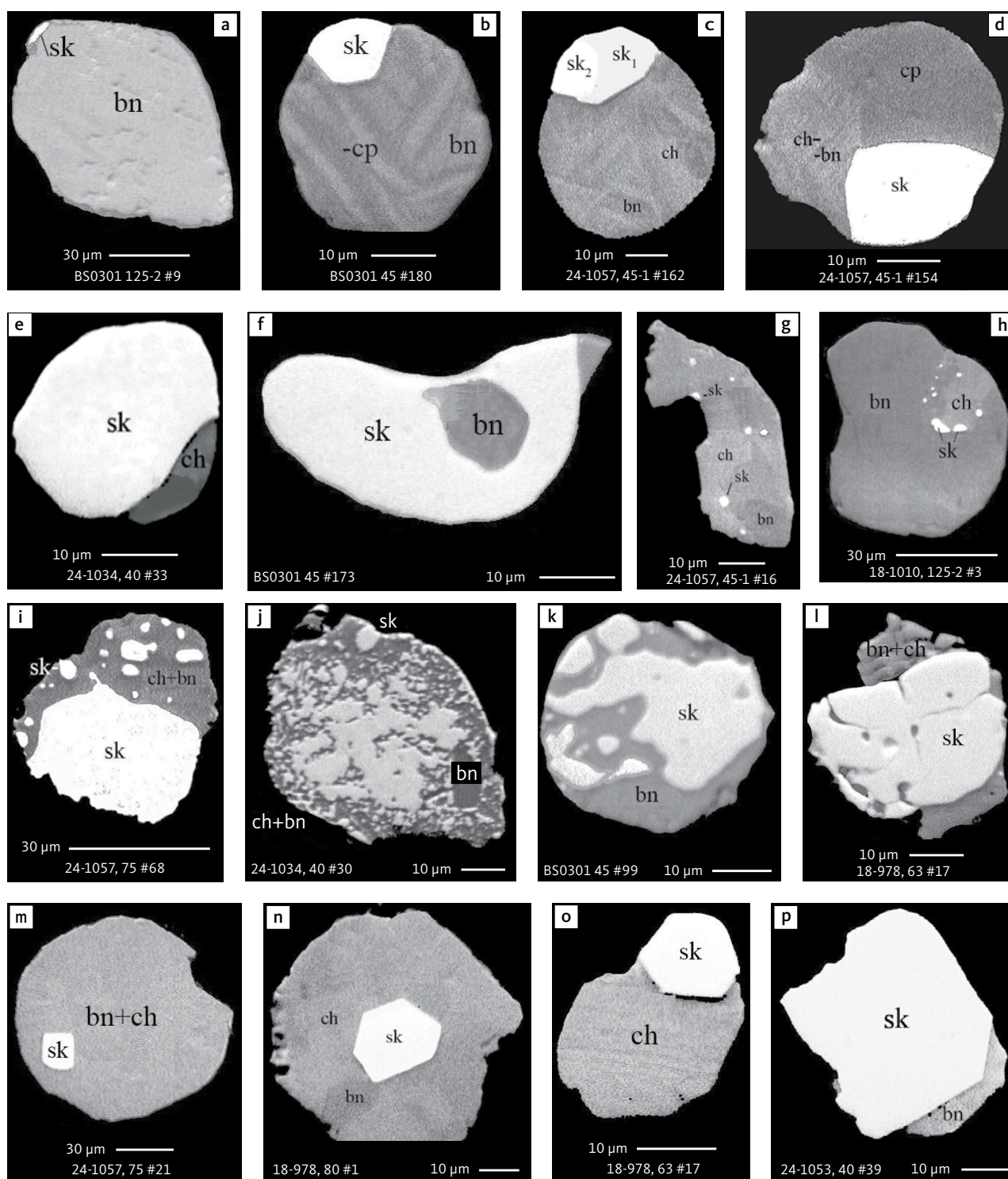
Fig. 16 BSE images showing the petrographic relations between skaergaardite and Cu-Fe sulphides in polished monolayer thin sections of HS concentrates. Table 3 provides formulae for the precious metal minerals. Formulae for common rock-forming minerals and base metal sulphides are found in Appendix 1. Note the multitude of relations from crystals of skaergaardite in centres as well as at margins of sulphide droplets, to a wide range of exsolution textures, and to tiny, disseminated droplets of skaergaardite throughout complex Cu-Fe sulphide grains. Abbreviated names of minerals, compounds and alloys are as follows: sk : skaergaardite including sk 1 : (PdCu) and sk 2 : (Pd,Au)Cu. bn : bornite; ch : chalcocite. cp : chalcocopyrite. Sample numbers and scales included in the images.
