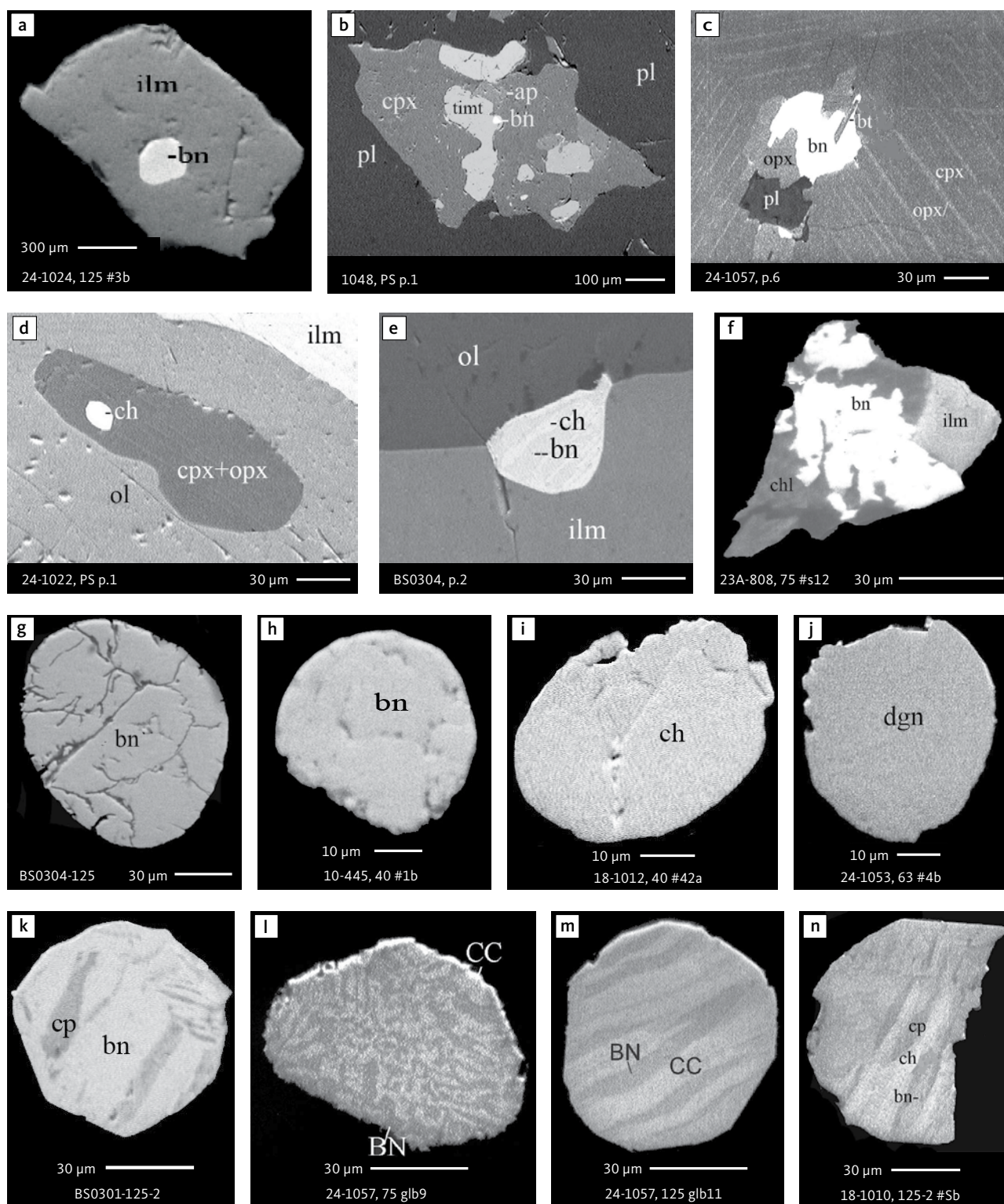
Fig. 7 BSE images of sulphides. Panels a-e are polished thin sections of gabbroic host. Panels f-n are polished monolayer thin sections of heavy mineral HS concentrates. Images include samples from the central part of the intrusion ( a-e, g-n ), and one sample from the marginal part of the intrusion ( f ). Note exsolution textures in panels k-n . Abbreviated names of minerals, compounds and alloys are as follows: bn and BN : bornite. ch and CC : chalcocite. cp : chalcopyrite. dgn : digenite. cpx : clinopyroxene. opx : orthopyroxene. pl : plagioclase. ol : olivine. timt : titaniferous magnetite. ilm : ilmenite. ap : apatite. bt : biotite. chl : chlorite. Grain numbers and scales included in the images. Table 3 provides formulae for the precious metal minerals. Formulae for common rock-forming minerals and base metal sulphides are found in Appendix 1.
