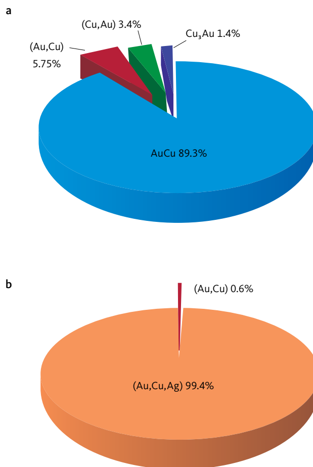
Fig. 22 Au-rich parageneses in a : mineralisation level Pd1/Au in all drill core samples from the centre of the intrusion and b : mineralisation level Pd4 near the margins of the intrusion. In (a), the average is based on data from samples 90-24-1018, 90-18-958 and bulk sample BS0304 from ToF (locations in Fig. 1) and is representative for the Au-rich levels in the central parts of mineralisation. In (b) the average is based on samples 90-23A-798 and 90-10-434. AuCu : tetra-auricupride; Cu 3 Au : auricupride; (Au,Cu) , (Cu,Au) , (Au,Cu,Ag) : alloys of Au, Cu and Ag. Not shown in (a): 0.1% unnamed compound Au 3 Cu and 0.1% (Au,Cu,Ag) alloy.
