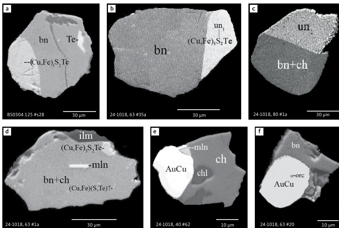
Fig. 9 BSE images of sulphides from the Au-rich Pd1/Au horizon in the central part of the intrusion. Polished monolayer thin sections of the heavy mineral HS concentrates. Table 3 provides formulae for the precious metal minerals. Formulae for common rock-forming minerals and base metal sulphides are found in Appendix 1. Formulae are given here for rare minerals that are not listed in Table 3 and Appendix 1. Abbreviated names of minerals, compounds and alloys are as follows: bn : bornite, ch : chalcocite, mln : melonite ( (\text{Ni,Pd})\text{Te}_2 ), Te : native tellurium, orc : orcelite ( \text{Ni}_{5-x}\text{As}_2 ), un 1 : unnamed compound (\text{Cu,Fe})_3\text{TeS}_2 , ilm : ilmenite, chl : chlorite. Grain numbers and scales included in the images.
