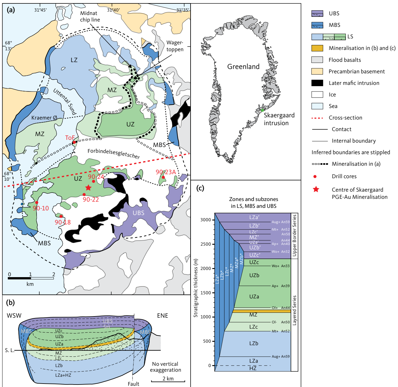
Fig. 1 Overview of the Skaergaard intrusion. a: Simplified geological map slightly modified from Nielsen et al. (2015, 2019a), showing the Layered Series (LS), the Marginal Border Series (MBS) and the Upper Border Series (UBS). The subzones of the LS include the Lower Zone (LZ), Middle Zone (MZ), and Upper Zone (UZ). In red, the collar locations for drill cores 90-10, 90-18, 90-23A and sampling site 'Toe of Forbindelsesgletscher' (ToF). b: WSW-ENE section (red stippled line in (a)) through the intrusion with subdivisions as in (a), and subzones a, b and c in LZ and UZ. c: Correlation between zones and sub-zones of LS, MBS and UBS (modified from Salmonsén & Tegner 2013).
