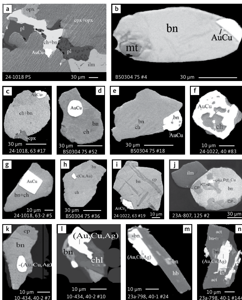
Fig. 23 BSE images showing the petrographic relations between (Au,Cu) phases and rock-forming minerals of the gabbroic host and sulphides. a : polished thin section of gabbro with interstitial sulphide and tetra-auricupride (AuCu). b–n : polished monolayer thin sections of HS concentrates. Panels a–i are from samples in the central part of the intrusion, and j–n are from samples near the margins of the intrusion. Table 3 provides formulae for the precious metal minerals. Formulae for common rock-forming minerals and base metal sulphides are found in Appendix 1. Grain numbers and scales included in the images. Abbreviated names of minerals, compounds and alloys are as follows: AuCu : tetra-auricupride. (Cu,Au) , (Au,Cu,Ag) : alloys of Au, Cu and Ag. (Au,Pd) 3 Cu : unnamed Au 3 Cu. kt : kotulskite (PdTe). bn : bornite. ch : chalcocite. cp and CP : chalcopyrite. opx : orthopyroxene. cpx : clinopyroxene. pl : plagioclase. ilm : ilmenite. hb : hornblende. act : actinolite. kth : keithconnite. mt : magnetite. chl : chlorite.
