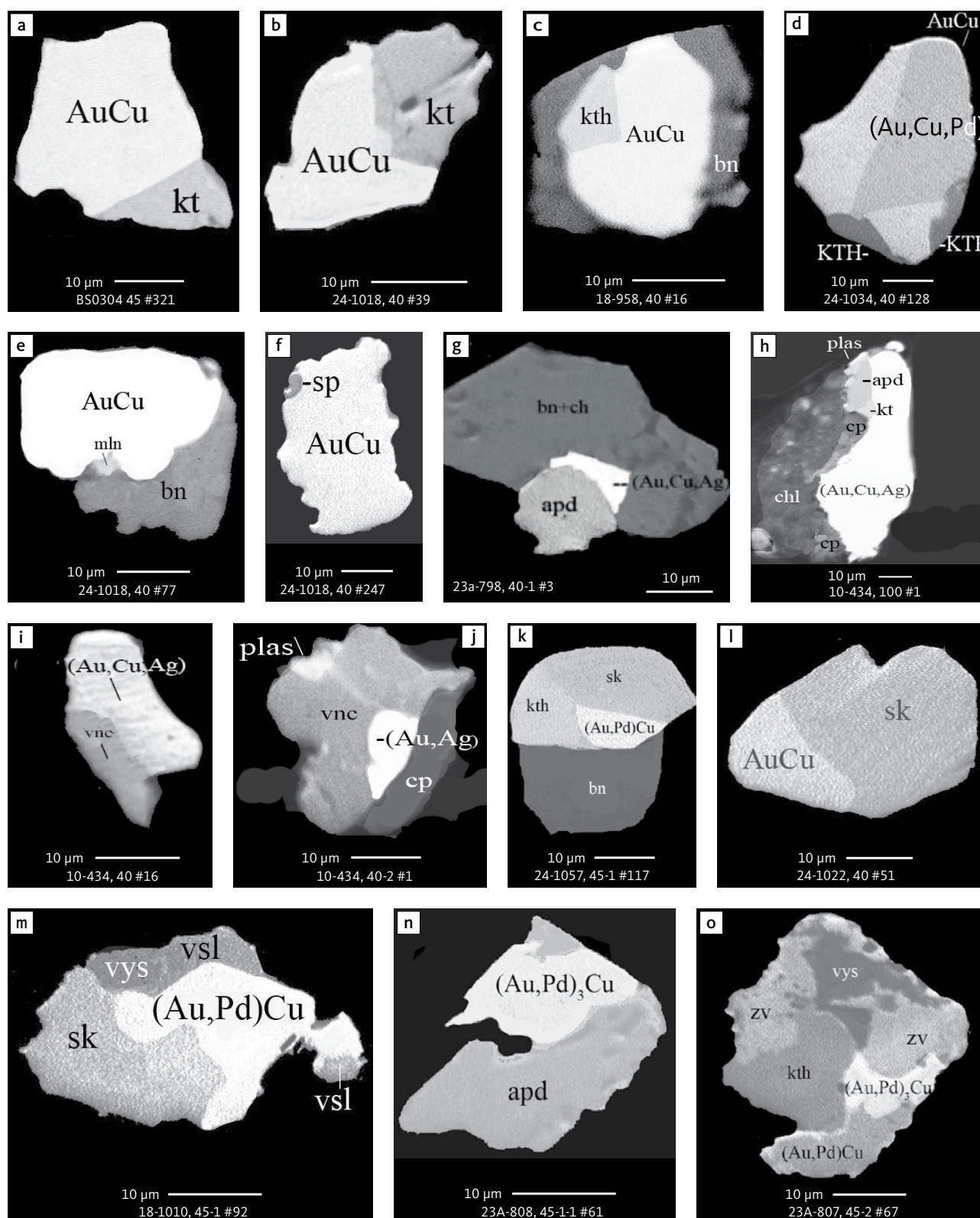
Fig. 26 BSE images of the petrographic relations between Au minerals and Cu minerals with PGEs in polished monolayer thin sections of the heavy mineral HS concentrates. The Au and Cu minerals are associated with virtually all other precious metal phases of the mineralisation. Table 3 provides formulae for the precious metal minerals. Formulae for common rock-forming minerals and base metal sulphides are found in Appendix 1. Grain numbers and scales included in the images. Abbreviated names of minerals, compounds and alloys are as follows: AuCu : tetra-aurocupride. (Au,Pd)Cu : tetra-aurocupride. (Au,Pd) 3 Cu : unnamed compound. (Au,Cu,Pd) , (Au,Cu,Ag) : alloys of Au, Cu, Pd and Ag. (Au,Ag) : native gold. sk : skaegeardite (PdCu). kt : kotulskite (PdTe). kth and KTH : keithconite (Pd 3 Te). mln : melonite (NiTe 2 ). sp : sperrylite. apd : arsenopalladinite. plas : palladoarsenide. vnc : vinctentite. vvs : vysotskite. vsl : vasillite. zv : zvyagintsevitte. bn : bornite. ch : chalcocite. cp : chalcopryite. chl : chlorite.
