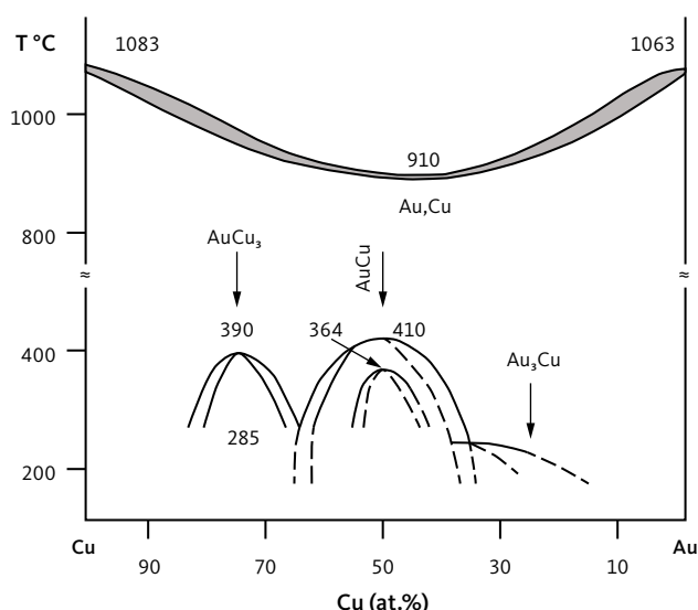
Fig. 35 Binary phase diagram for Au-Cu (Savitsky 1984; Okamoto et al. 1987) showing the stability fields of phases with falling temperature. All these phases have been found in the HS concentrates from the Skaergaard PGE-Au Mineralisation. Grey shading: temperature range for liquidus to solidus transition for (Cu,Au) alloy. Solid lines: established boundaries of stability fields. Dashed lines: approximate positions of the boundaries. Boundaries at lower temperatures separate structural types of (Cu,Au) alloys stable at decreasing temperature (see Okamoto et al. 1987 for details).
