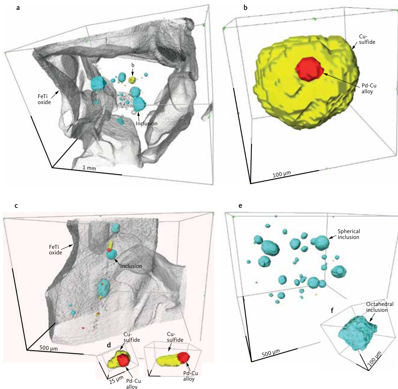
Fig. 15 Recompiled High-Resolution X-ray Computed Tomography (HRXCT) images after Godel et al. (2014) showing 3D images of the relationship between FeTi oxides (grey), Cu-, and Fe-sulphides (yellow), skagaardite (red) and silicate inclusions (blue) enclosed in FeTi oxides. a: View into an ilmenite grain with silicate inclusions and sulphide droplet with skagaardite grain attached. b: Magnified image of the sulphide droplet. c: Trains of silicate and sulphide with skagaardite, possibly along pathway for interstitial melt. d: Focussed view shows the high skagaardite to sulphide ratio compared to the ratio for sulphide droplets enclosed in ilmenite. e: Focussed view of the perfectly spherical inclusions with hydrous silicates and the octahedral inclusion rich in FeTi oxides. The latter, also referred to as negative crystals, formed from silicate melt that was trapped while the ilmenite host crystallised.
