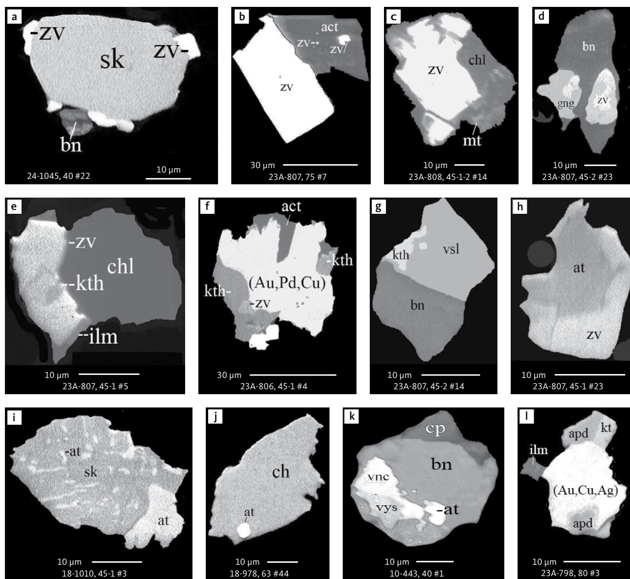
Fig. 30 BSE images of Pd, Cu and Ag intermetallic compounds with Pb, Te, Sn, Sb and Bi in polished monolayer thin sections of HS concentrates. Zvyagintsevite ( \text{Pd}_3\text{Pb} ) is the dominant Pd phase in samples from the eastern margin, commonly in association with actinolite. Table 3 provides formulae for the precious metal minerals. Formulae for common rock-forming minerals and base metal sulphides are found in Appendix 1. Abbreviated names of minerals, compounds and alloys are as follows: zv : zvyagintsevite. kth : keithconnite. kt : kotulskite. vnc : vinctite. gng : guanglinite (obsolete and renamed to vinctite). apd : arsenopalladinite. at : atokite. sk : skaergaardite. vys : vysotskite. vsl : vasilite. (Au,Pd,Cu) and (Au,Cu,Ag) : alloys Au, Cu and Pd. bn : bornite. cp : chalcopyrite. ch : chalcocite. ilm : ilmenite. mt : magnetite. act : actinolite. chl : chlorite. Grain numbers and scales included in the images.
