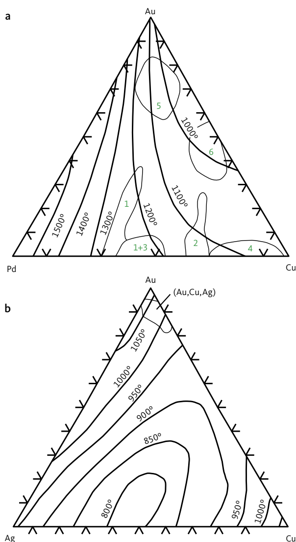
Fig. 33 Phase diagrams showing compositions (wt%) of a : primary Cu, Pd and Au and b : primary alloys of Au, Cu and Ag on experimental liquidus surfaces of the Au-Cu-Pd system (°C; after Savitsky (1984). Compositional fields shown in (a) for the Au-Cu-Pd system are as follows: 1 : skaergaardite. 2 : nielsenite ( \text{Cu}_3\text{Pd} ). 3 : (\text{Pd,Cu})_\beta alloys. 4 : (\text{Cu,Pd})_\alpha alloys. 5 : (\text{Au,Cu,Pd}) alloys. 6 : (\text{Au,Cu,Ag}) alloys. Compositional field shown in (b) for the Au-Cu-Ag system includes (\text{Au,Cu,Ag}) alloys.
