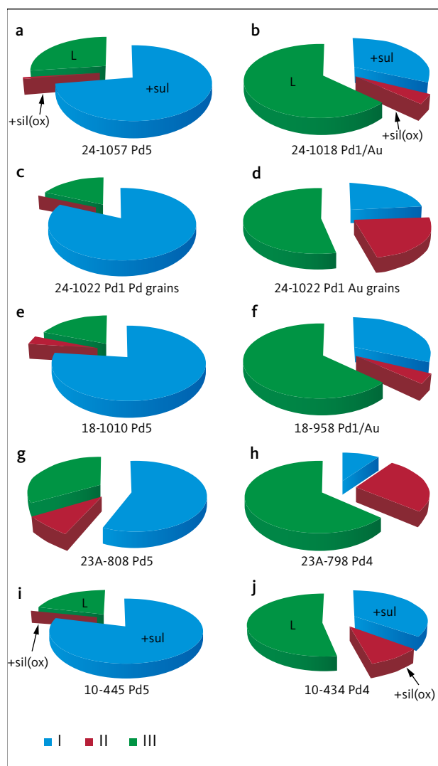
Fig. 37 Petrographic associations of precious metal mineral grains in individual samples (1 m intervals) from the lower PGE-rich (Pd5) mineralisation level and the Au-rich upper mineralisation levels (see Chapter 2) in \sim 125 \mu\text{m} powders. Samples are identified by the unique number of the drill core followed by the depth in the core from where the sample was collected. E.g. sample 24-1057 collects the interval between 1057 and 1058 m in drill core 90-24. The precious metal phases are as follows: I : attached to sulphides ( +sul ), II : attached to silicates and FeTi oxides ( +sil(ox) ) or III : as liberated grains ( L ). Proportions of I to III are normalised to 100% and include data from drill cores 90-10, 90-18, 90-23A and 90-24 (Table 22). In the PGE-rich layer (Pd5) the precious metal minerals are associated with sulphides and occur as free phases with only small proportions associated with silicates and FeTi oxides. Conversely, the precious metal grains in the Au-rich mineralisation levels occur mostly as free grains but with high and variable proportions associated with either silicates and FeTi oxides or sulphides.
