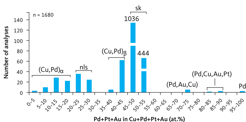
Fig. 11 Intermetallic compounds and alloys ranging from Cu to Pd. Based on EMP analyses of a total of 1680 grains. Minerals, compounds and alloys are identified on the basis of precious metal to Cu ratio expressed as (Pd+Au+Pt) in at.%. From left to right: (Cu,Pd) α alloy: 3–20 at.%; nls: nielsenite (PdCu 3 ), 20–30 at.%; (Cu,Pd) β alloy: 35–45 at.%; sk: skaergaardite (PdCu), 45–55 at.%; (Pd,Au,Cu) solid solution: 70–75 at.%; (Pd,Cu,Au,Pt) solid solution: 80–90 at.%; Pd: native Pd, c. 100 at.%. Note that bars for “sk” are shortened to fit the diagram.
