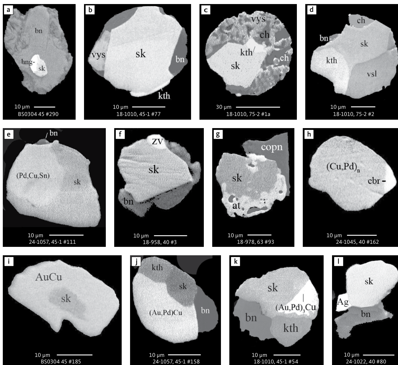
Fig. 19 BSE images showing the relationship between Cu and Pd minerals and other precious metal minerals in polished monolayer thin sections of HS concentrates. Table 3 provides formulae for the precious metal minerals. Formulae for common rock-forming minerals and base metal sulphides are found in Appendix 1. Note the high proportions of precious metal to Cu-Fe sulphide and in the rimming of skagaardite by tetra-aurocupride in panel i. Abbreviated names of minerals, compounds and alloys are as follows: sk : skagaardite. (Cu,Pd) n : alloy of Cu and Pd. hng : hongshiite (Pt,Pd,Au) (Cu,Fe). vys : vysotskite. vsl : vasilite. at : atokite. kth : keithconnite. zv : zvyagintsevite. cbr : cabriite. (Pd,Cu,Sn) : alloys of Pd, Cu and Sn. AuCu and (Au,Pd) 3 Cu : tetra-aurocupride. (Au,Pd) 3 Cu : unnamed compound. Ag : native silver. bn : bornite. ch : chalcocite. copn : cobaltian pentlandite. Grain numbers and scales included in the images.
