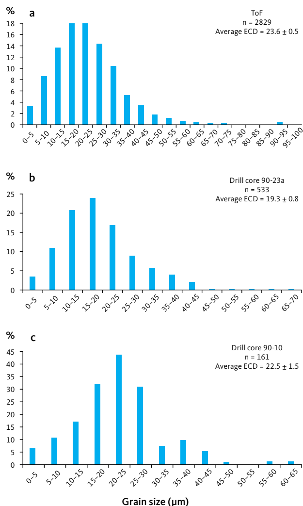
Fig. 36 Variation in grain size ( \mu\text{m} ) of precious metal grains in a : central part of the mineralisation (ToF: Toe of Forbindelsesgletscher), b : drill core 90-23A near the eastern margin and c : drill core 90-10 near the western margin. The central part of the mineralisation shows a relatively small increase in grains >30 \mu\text{m} .
