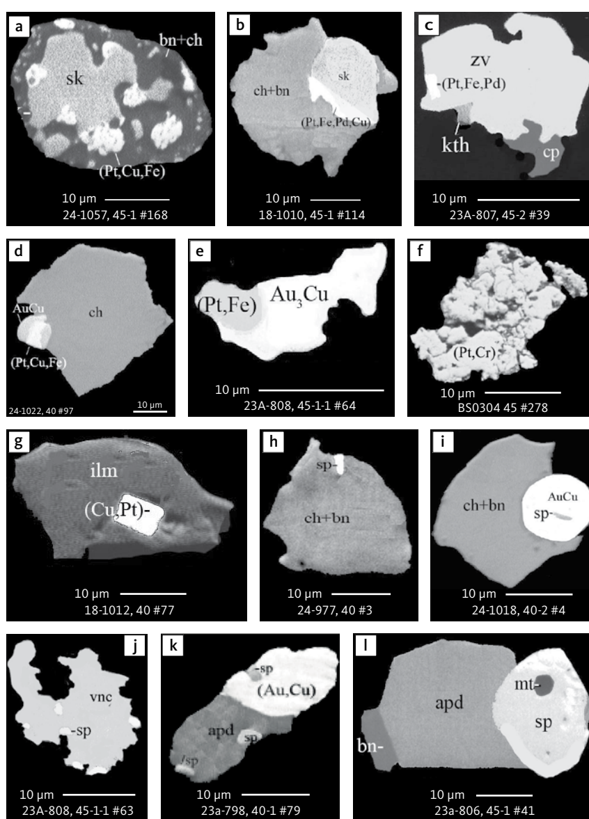
Fig. 20 BSE images of Pt minerals in polished monolayer thin sections of HS concentrates. Table 3 provides formulae for the precious metal minerals. Formulae for common rock-forming minerals and base metal sulphides are found in Appendix 1. Abbreviated names of minerals, compounds and alloys are as follows: (Pt,Cu,Fe), (Pt,Fe,Pd,Cu), (Pt,Fe,Pd), (Pt,Fe), (Cu,Pt): alloys of Pt, Cu, Fe, and Pd. (Pt,Cr): alloys of Pt and Cr. (Au,Cu): alloys of Au and Cu. sp: sperrylite. sk: skaergaardite. zv: zvyagintsevite. kth: keithconnite. apd: arsenopalladinite. vnc: vincentite. AuCu: tetra-auricupride. Au 3 Cu: unnamed compound. bn: bornite. ch: chalcocite. cp: chalcopyrite. ilm: ilmenite. mt: magnetite. Grain numbers and scales included in the images.
