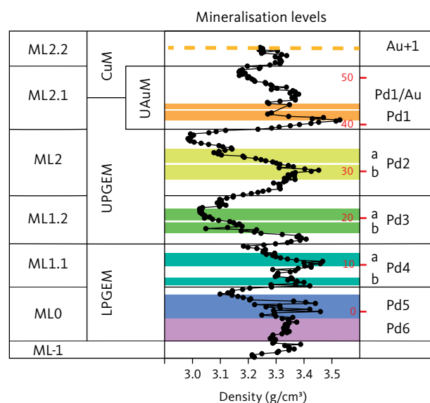
Fig. 3 Summary of the Skaergaard mineralisation. From left to right: macrorhythmic layers (ML-1 to ML2.2); geochemical subdivisions of the mineralisation, includes the Lower PGE Mineralisation (LPGEM), Upper PGE Mineralisation (UPGEM), Upper Au Mineralisation (UAuM) and Cu Mineralisation (CuM, see Nielsen et al. 2015 for detailed explanations); density (g/cm³) of bulk rocks and mineralisation levels from centrally-located drill cores; and mineralisation levels (Pd6 and Pd5 in ML0, Pd4a, b in ML1.1, Pd3a, b in ML1.2, Pd2a, b in ML2 and Pd1 and Pd1/Au in ML2, and Au+1 in ML2.1). Au+1 (stippled orange line) is only found in drill core 90-18. This concordant mineralisation level is Cu-rich and poor in precious metals in all other drill cores. The PGE peak in Pd5 (designated 0 m in the mineralisation) provides a marker throughout the intrusion (Nielsen et al. 2015; Fig. 4a). The correlations in the 15–40 m succession of mineralisation levels are based on systematic assays in Watts, Griffiths & McQuat Ltd (1991). Figure modified from Nielsen et al. (2015, 2019a).
