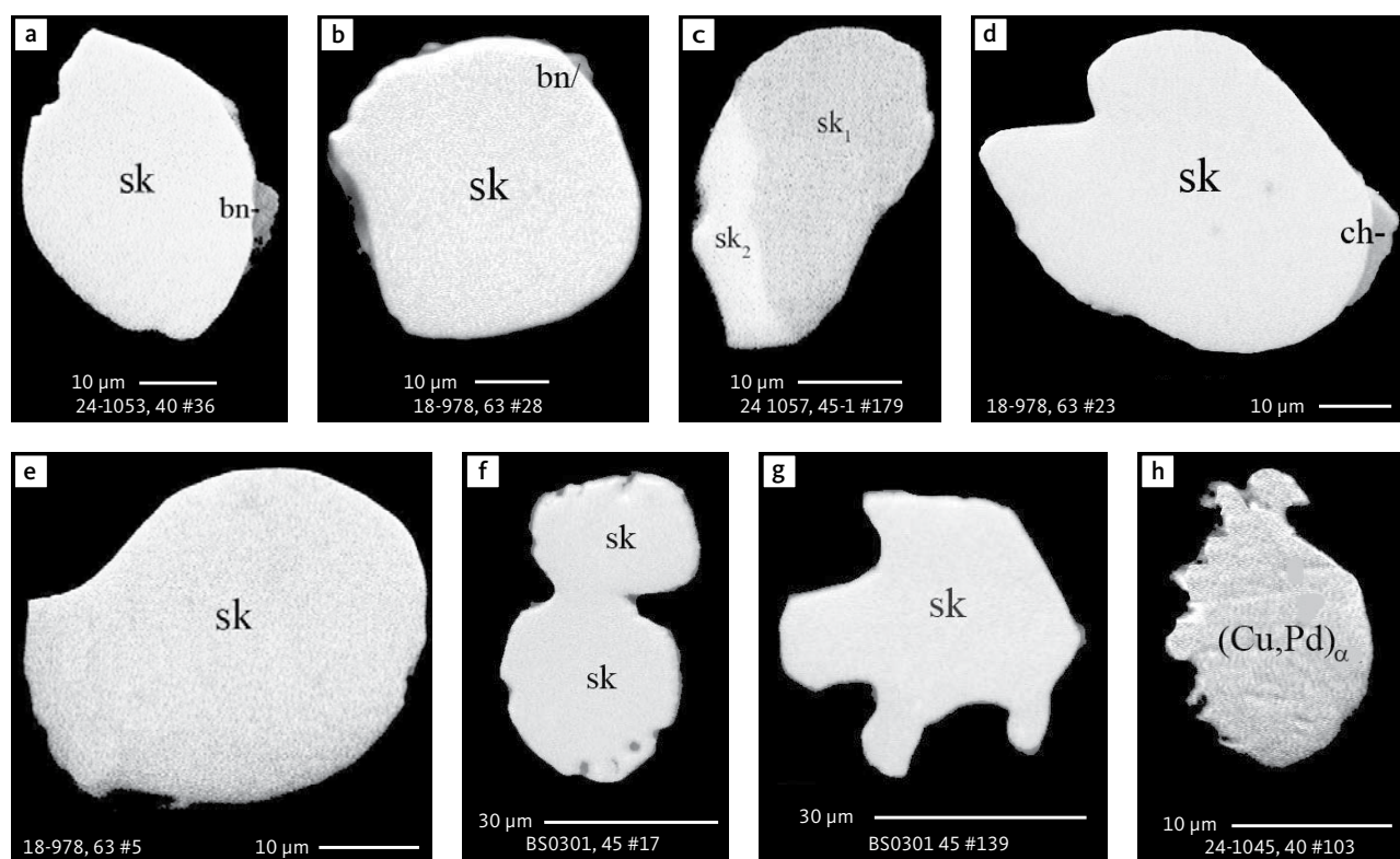
Fig. 18 BSE images of free grains of Cu and Pd minerals in polished monolayer thin sections of HS concentrates. The rounded grains may be droplets or grains formed during exsolution in sulphide (E. Makovicky, pers. comm. 2008). Note the grain in panel f, which appears to have formed by amalgamation of two individual grains. Abbreviated names of minerals, compounds and alloys are as follows: sk : skaergaardite (PdCu) including sk 1 : (PdCu) and sk 2 : ((Pd,Au)Cu). (Cu,Pd) α : unnamed alloy. ch : chalcocite. bn : bornite. Table 3 provides formulae for the precious metal minerals. Formulae for common rock-forming minerals and base metal sulphides are found in Appendix 1. Grain numbers and scales included in the images.
