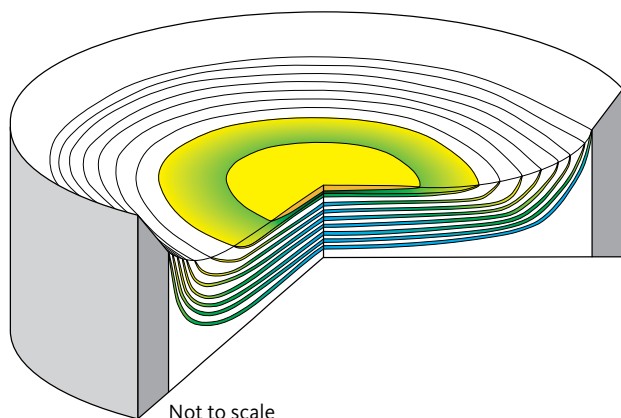
Fig. 5 Visualisation of the 3D structure of the precious metal-rich part of the mineralisation (not to scale). The stack of PGE-rich mineralisation levels with upward-decreasing diameter within the bowl-shaped succession of macrorhythmic layers. Blue shading: PGE-rich; green shading: Au-rich; yellow shading: Au-rich but PGE-poor layers. The maximum concentration of Au is in the uppermost mineralisation level in the central part of the intrusion. Modified from Nielsen et al. (2019a).
