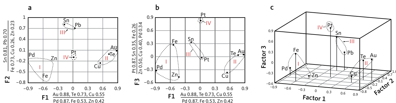
Fig. 12 Factor analysis on the skaergaardite (PdCu) composition from sample 90-24-1057 in level Pd5. A total of 311 analyses are included in the modelling. a: F1 (factor 1) versus F2 (factor 2). b: F1 (factor 1) versus F3 (factor 3). c: 3D diagram of all three factors. The compositions indicated by the stippled lines include group I: (Pd-Fe-Zn); group II: (Cu-Au-Te); group III: (Pb-Sn); group IV: Pt-rich skaergaardite. Modified from Rudashevsky et al. (2004).
