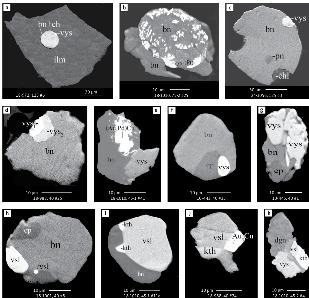
Fig. 28 BSE images of vysotskite and vasilite in polished monolayer thin sections of HS concentrates. The precious metal sulphides form as exsolutions in sulphide droplets, as exsolutions on the margins of sulphide globules and as irregular grains intergrown with other precious metal phases. Table 3 provides formulae for the precious metal minerals. Formulae for common rock-forming minerals and base metal sulphides are found in Appendix 1. Grain numbers and scales included in the images. Abbreviations: vys : vysotskite, including Pd-rich vys 1 and Pt-rich vys 2 . vys-(Pt) : vysotskite with no Pt. vsl : vasilite. kth : keithconnite. (Au,Pd)Cu : tetra-aurocupride. Au 3 Cu : unnamed compound. bn : bornite. ch : chalcocite. cp : chalcocopyrite. dgn : digenite. pn : pentlandite. ilm : ilmenite. chl : chlorite.
