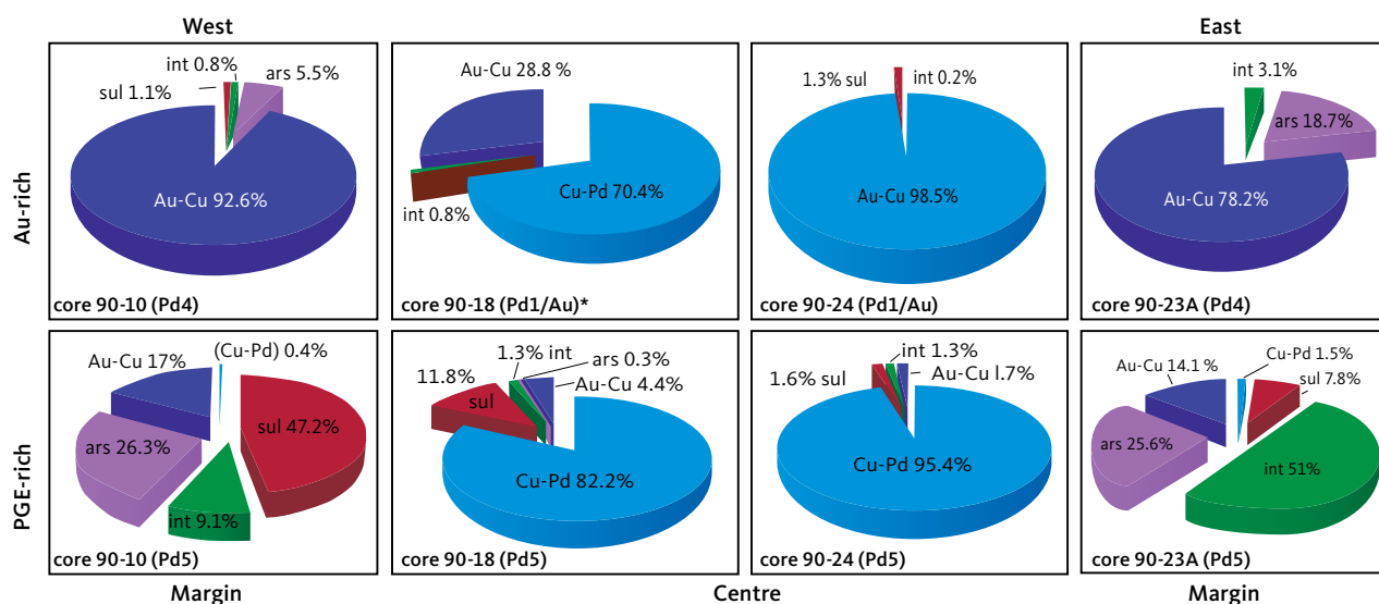
Fig. 10 Contrasts between precious metal parageneses across the intrusion in the upper Au-rich mineralisation and the lower PGE-rich mineralisation level (Pd5). The data are summarised for drill cores 90-10 near the western margin, 90-18 from the SW centre, 90-24 from the centre, and 90-23A near the eastern margin (drill core locations in Fig. 1; original data in electronic appendix 12 of Nielsen et al. 2019a). The lower PGE-rich levels are perfectly concordant with variations in Pd/Pt ratios up the layered gabbros despite the stark contrasts in parageneses. The Au-rich mineralisation levels are found increasingly higher in the succession of gabbro layers towards the centre of the intrusion (see also Fig. 4). The Au-rich mineralisation levels are Pd1/Au in core 90-24, Pd1/Au* and in Au+1 in 90-18 and Pd4a in cores 90-10 and 90-23A. Total areas of precious metals are recalculated to 100% and used as approximations to volume relations. Cu-Pd : minerals, intermetallic compounds and alloys of Cu and Pd that may be substituted by Pt, Fe, Cu and/or Cr; Au-Cu : minerals, intermetallic compounds and alloys of Au and Cu (Ag); sul : sulphides of Pd, Cu (Ag, Cd, Hg, Ti); ars : arsenides of Pd (Pt, Ni); int : intermetallic compounds of Pd, Cu, Sn, Pb, Te (Co, Sb, Bi).
