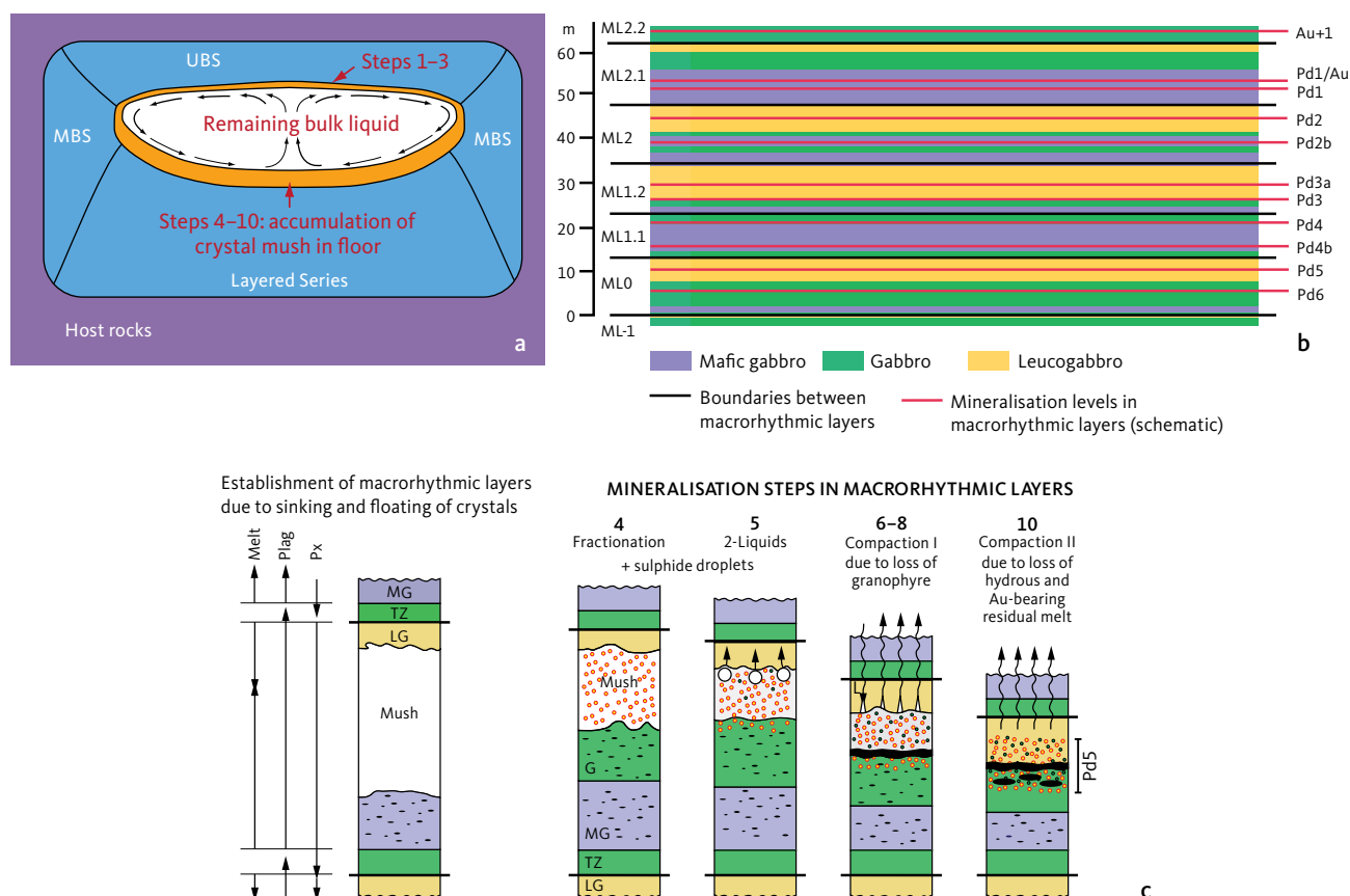
Fig. 38 Summary of the mineralisation processes in the Skaergaard PGE-Au Mineralisation, as developed in Nielsen (2016) and Nielsen et al. (2015, 2019a, b). a : Trapping and accumulation of precious metals ( steps 1-3 ) during which the precious metals are brought to the floor mush (based on fig. 26 in Nielsen et al. 2015). Blue : solidified gabbro. Orange : mush zones with trapping. White : remaining bulk liquid. Purple : Palaeogene and Precambrian host rocks. Red arrows point to the zone of trapping of precious metals under the roof ( steps 1-3 ) and the crystallisation and mineralisation processes in the floor mush ( steps 4-10 ). b : Correlation between mineralisation levels and the macrorhythmic layers. The bowl shape of the layers is omitted for clarity. The lower four macrorhythmic layers host two mineralisation levels each, including a lower level due to density accumulation and an upper level due to in situ sulphide saturation in residual Fe-rich mush melt (based on fig. 8 in Nielsen et al. 2015 and fig. 5 in Nielsen et al. 2019a). c : Upward accumulation, fractionation and transport of the precious metals in mush melts. Steps 4-10 within ML0 macrorhythmic layer hosts the main PGE-mineralisation level, Pd5. Sinking of dense phases and the rise of plagioclase in the proto-macrorhythmic layers allowed mush melt to evolve in between the two. Sulphide saturation is reached due to crystallisation and fractionation of the mush melt ( yellow dots with red rims ) and is followed by silicate immiscibility ( blue dots with black rims ), and loss of Si-rich conjugate melt, ponding of dense Fe-rich silicate melts and subsequently the loss of the residual Fe-rich silicate melt and free volatile phase. Steps 4-10 are repeated in all mineralisation layers from ML0 to ML2.1 (based on fig. 22 in Nielsen et al. 2015). MBS : Marginal Border Series. UBS : Upper Border Series. ML-1 to ML2.2 : macrorhythmic layers. Plag : plagioclase. Px : pyroxene. MG : melagabbro. G : gabbro. LG : leucogabbro. TZ : transitional zone.
