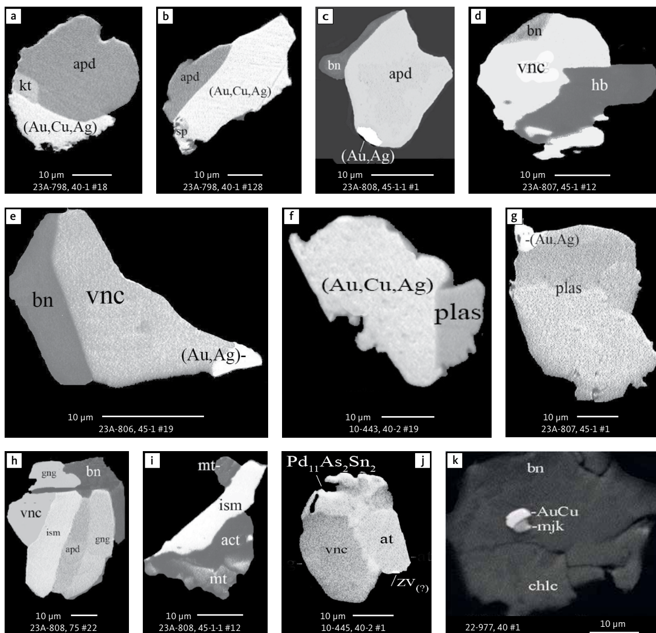
Fig. 32 BSE images of PGE arsenides in polished monolayer thin sections of HS concentrates. As for the intermetallic compounds (see text and Fig. 31), arsenides are related to a wide range of precious metal phases and sulphides, while local geochemical balances control the parageneses. Table 3 provides formulae for the precious metal minerals. Formulae for common rock-forming minerals and base metal sulphides are found in Appendix 1. Formulae are given here for rare minerals or compositional varieties that are not listed in Table 3 or Appendix 1. Abbreviated names of minerals, compounds and alloys are as follows: apd : arsenopalladinite/stillwaterite ( \text{Pd}_3\text{As}_3 ). kt : kotulskite. sp : sperrylite. vnc : vincentite. gng : guanglinite (obsolete and renamed to vincentite). plas : palladoarsenide. ism : isomertiete ( \text{Pd}_{11}\text{As}_2(\text{Sb},\text{Sn})_2 ). mjk : majakite. zv : zvyagintsevite. at : atokite. \text{Pd}_{11}\text{As}_2\text{Sn}_2 : unnamed compound. AuCu : tetra-auricupride. (Au,Cu,Ag) : alloys dominated by Au and Cu. (Au,Ag) : native gold. bn : bornite. chlc : chalcocite. hb : hornblende. act : actinolite. mt : magnetite. Grain numbers and scales included in the images.
