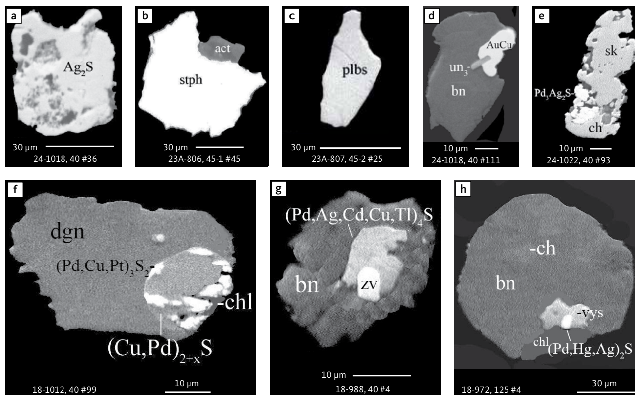
Fig. 29 BSE images of rare PGE sulphides in polished monolayer thin sections of HS concentrates. All phases are rare and some are found only as single grains. Table 3 provides formulae for the precious metal minerals. Formulae for common rock-forming minerals and base metal sulphides are found in Appendix 1. Formulae are given here for rare minerals that are not listed in Table 3 or Appendix 1. Abbreviated names of minerals, compounds and alloys are as follows: AuCu : tetra-auricupride. Ag 2 S : acanthite/argentite. stph : stephanite (Ag 5 SbS 4 ). plbs : polybasite (Ag 16 Sb 2 S 11 ). Pd 3 Ag 2 S : coldwellite. sk : skaergaardite. un 3 : unnamed compounds, including (Pd 3 Cu 6 S 3 Te 2 ), (Pd,Hg,Ag) 2 S, (Cu,Pd) 2+x S, (Pd,Cu,Pt) 3 S 2 and (Pd,Ag,Cd,Cu,Tl) 4 S. zv : zvyagintse-vite. vys : vysotskite. bn : bornite. ch : chalcocite. dgn : digenite. act : acanthite. chl : chlorite. Grain numbers and scales included in the images.
