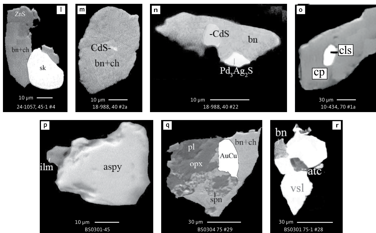
Fig. 8 (Continued) BSE images of rare minerals in polished monolayer thin sections. Table 3 provides formulae for the precious metal minerals. Formulae for common rock-forming minerals and base metal sulphides are found in Appendix 1. Formulae are given here for rare minerals that are not listed in Table 3 or Appendix 1. Abbreviated names of minerals, compounds and alloys are as follows: copn and pn-(Co) : cobaltian pentlandite (panels a–d). pn : pentlandite (panels e–f). po : hexagonal pyrrhotite (panel g). gn : galena (panels h–j). sph : sphalerite (panel k). ZnS : sphalerite (panel l). CdS : greenockite/hawleyite (panels m, n). cls : clausthalite ( \text{PbSe} ) (panel o). aspy : arsenopyrite (panel p). spn : thiospinel group, carrollite ( \text{Cu}(\text{Co}, \text{Fe}, \text{Ni})_2\text{S}_4 ) (panel q). atc : atacamite ( \text{Cu}_2\text{Cl}(\text{OH})_3 ) (panel r). sk : skargaardite (panels a, b, e, g, l). (Cu,Pd) : Cu-Pd alloy (panel c). nls : nielsenite ( \text{PdCu}_3 ) (panel c). at : atokite ( \text{Pd}_3\text{Sn} ) (panel e). AuCu : tetra-auricupride (panels f, q). (Au,Ag) : native gold (panel h). \text{Pd}_3\text{Ag}_2\text{S} : coldwellite (panel n). vsl : vasilite ( (\text{Pd}, \text{Cu})_{16}\text{S}_7 ) (panel r). bn : bornite. ch : chalcocite. cp : chalcopyrite (panels h, o). cpx : clinopyroxene (panel j). opx : orthopyroxene (panels j, q). pl : plagioclase (panel q). ilm : ilmenite (panels i, p). sk : skargaardite (panel l). Grain numbers and scales included in the images.
