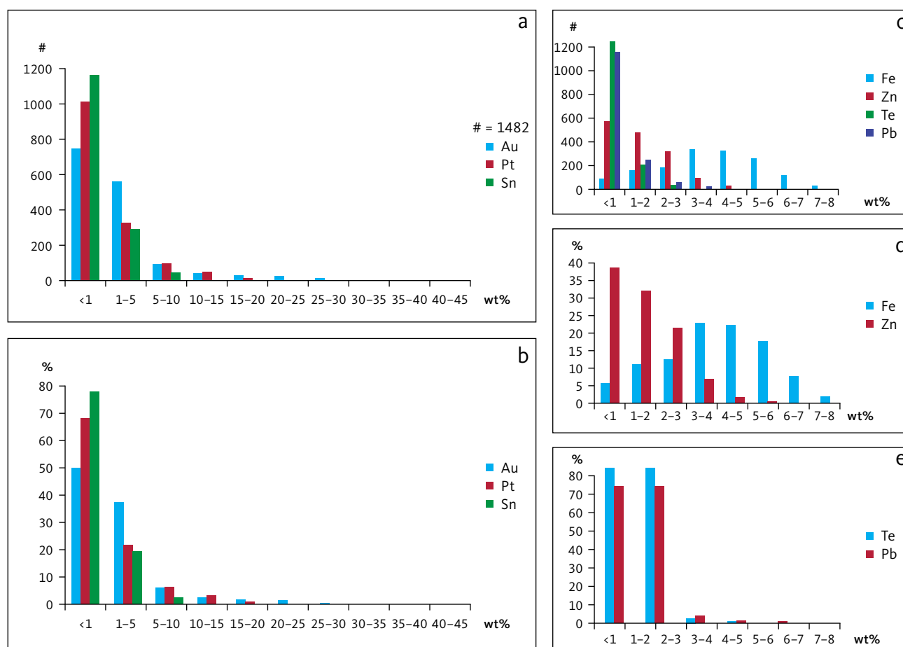
Fig. 13 Histograms illustrating frequency of substitutions in skaergaardite based on a total of 1482 EMP analyses. a: Au, Pt, Sn substitutions vs. number of analyses (#). b: Au, Pt, Sn substitutions vs. frequency (f) in %. c: Fe, Zn, Te, Pb substitutions vs. number of analyses. d: Fe and Zn substitutions vs. frequency. e: Te and Pb substitutions vs. frequency.
