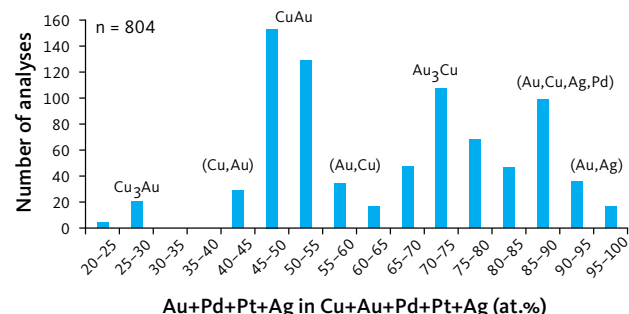
Fig. 21 Compositions and proportions of Au-Cu minerals and phases. The histogram shows the wide compositional range and the frequency of Au-rich minerals, intermetallic compounds and alloys of Au and Cu in the mineralisation. Based on compositions of a total of 804 analyses and expressed as sum of (Au+Pd+Pt+Ag) in at.%. The data set includes 0.1% unnamed compound Au 3 Cu and 0.1% (Au,Cu,Ag) alloy, which are not shown here. Abbreviations are as follows: CuAu : tetra-aurocupride. Cu 3 Au : aurocupride. (Au,Cu) , (Cu,Au) , (Au,Cu,Ag,Pd) : alloys of Au, Cu and Ag.
