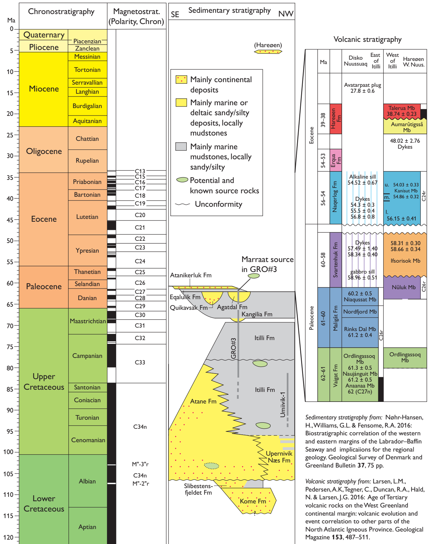
Fig. ES1. Stratigraphic summary of the Nuussuaq Basin.
